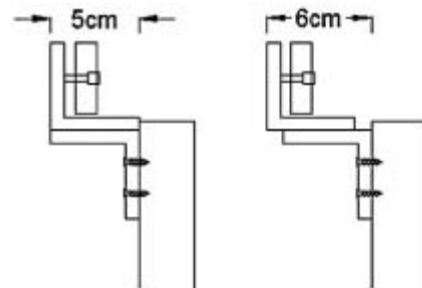
ADJUSTMENT INSTALLATION OF L-Z BRACKETS
