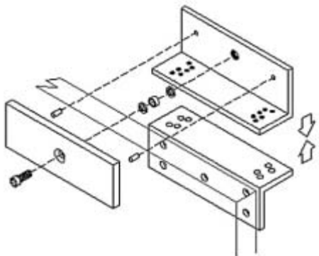
INSTALLATION OF L-Z BRACKETS
